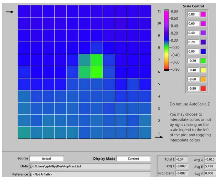
FIGURE 4. Segmented cell data showing the spatially resolved performance effect of a 1\ \text{cm}^2 bare spot in the anode at a total cell current density of 1.2\ \text{A}/\text{cm}^2 . The color scale shows the difference in local current performance between the defected cell and a pristine cell. The cell is operated at anode/cathode conditions of 100/50% relative humidity, 150/150 kPa, 1.5/2.0 stoich, hydrogen/air, and a cell temperature of 80^\circ\text{C} .
