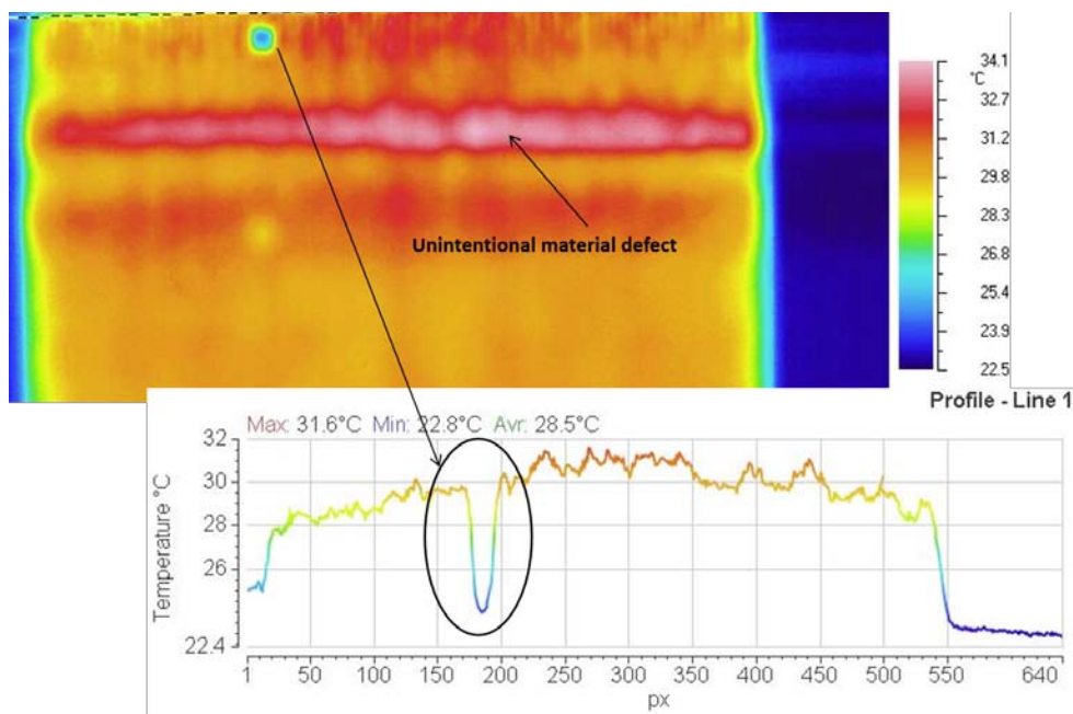
FIGURE 1. IR/RIF data from web-line demonstration, showing detection of a 0.25 cm 2 defect having a 100% reduction in the nominal electrode thickness (a bare spot), at a web speed of 30 fpm. The line graph of cross-web temperature shows the thermal response of this defect. Also shown on the image is indication of an unintentionally created band of thicker electrode coating.
