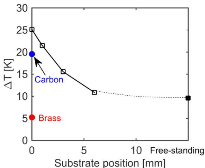
FIGURE 2. IR/RIF modeling result, showing predicted increase in the differential temperature created by a 5 mm electrode bare spot at 10 fpm web speed and 32.5 standard liter per minute jet velocity as a function of backing surface proximity to the back of the GDE.
