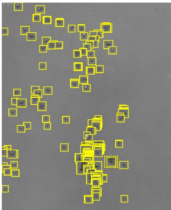
FIGURE 3. Optical reflectance image showing automated detection of particulates on electrode surface of GDE. The individual images of the particles inside the yellow boxes are magnified 10x.
