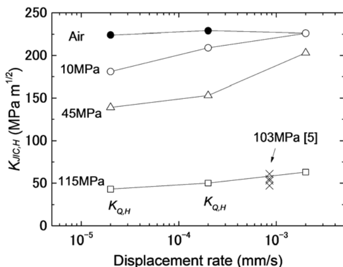
FIGURE 2. Rising-displacement fracture thresholds measured for SCM 435 pressure vessel steel in air and high-pressure hydrogen gas as a function of loading rate. The cross symbols are previous measurements performed at Sandia on a similar Cr-Mo pressure vessel steel (SA-372 Grade J) in 103 MPa hydrogen gas.
