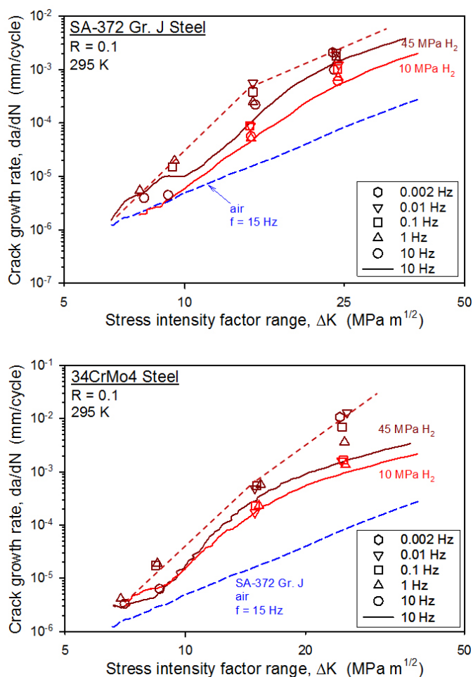
FIGURE 1. Composite data showing fatigue crack growth rate (da/dN) vs. stress-intensity factor range ( \Delta K ) and da/dN vs. frequency for two Cr-Mo pressure vessel steels in 10 MPa and 45 MPa hydrogen gas. The dark red dashed lines indicate corrections applied to the baseline da/dN vs. \Delta K relationships to reflect upper-bound behavior based on the da/dN vs. frequency data.
