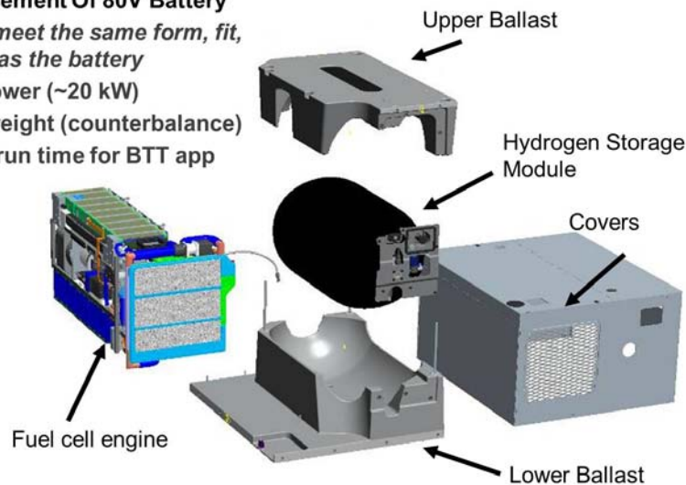
FIGURE 1. Direct replacement of 80-V battery
