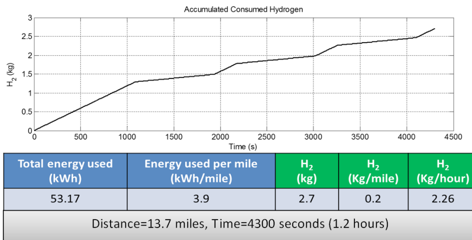
FIGURE 2. Performance data and energy efficiency and consumption for 24,500 kg refuse truck
