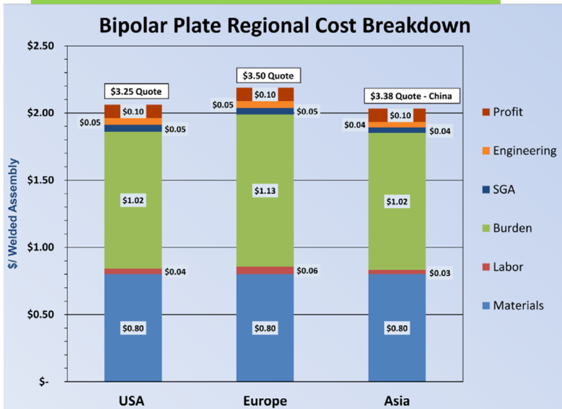
FIGURE 3. Regional cost breakdown for bipolar plates
