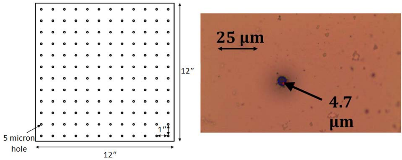
FIGURE 1. Schematic of a membrane calibration sheet and a microscope image of a laser machined hole
