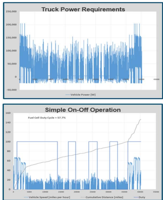
FIGURE 1. Simulated truck requirements
