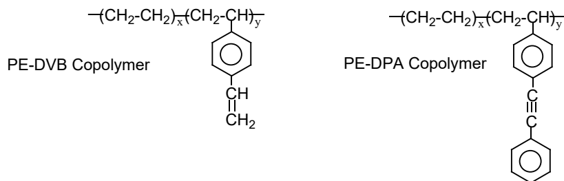
Scheme 2. Two reactive PE copolymers, including poly(ethylene-co-divinylbenzene) (PE-DVB) and poly(ethylene-co-vinylidiphenylacetylene) (PE-DPA)
