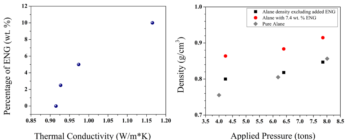
Figure 2. Thermal conductivity of SRNL alane with the addition of ENG at different weight % loadings (left) and density of alane at different applied pressures (right)
