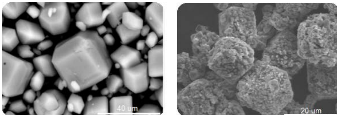
Figure 3. Scanning electron microscopy image of alane before and after desorption
