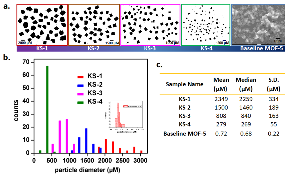
Figure 2. (a) Images and (b) plot of particle size distribution for five MOF-5 powders of varying particle sizes (KS-1 to KS-4, and baseline MOF-5). (c) Table of particle size range and median diameter for all samples.
