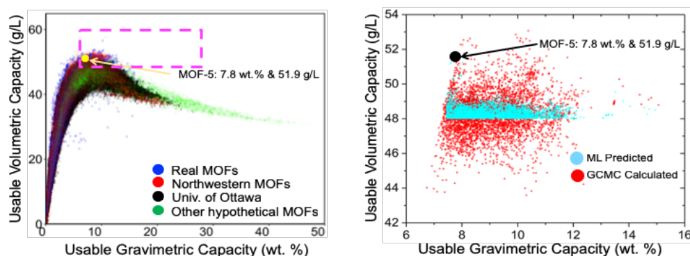
Figure 1. Verification calculations using GCMC on the top 4,847 MOFs predicted to be high-capacity materials by ML at temperature + pressure swing conditions between 100 bar at 77 K and 5 bar at 160 K. (a) Usable volumetric hydrogen storage capacity as a function of usable gravimetric capacity of 396,610 unseen MOFs (out of in total 495,305 MOFs excluding 98,695 compounds for which GCMC calculated capacities are available and used in training and testing ML models) predicted by ML. MOFs selected for further study by GCMC are shown by the pink dashed rectangular region; this includes MOFs with pressure swing capacities greater than or equal to 48 g/L and 7.5 wt %. (b) Usable volumetric hydrogen storage capacity as a function of usable gravimetric capacity for the 4,847 MOFs selected in panel a. For reference, the capacity of MOF-5 (7.8 wt % and 51.9 g/L), the highest capacity identified thus far, is also shown.
