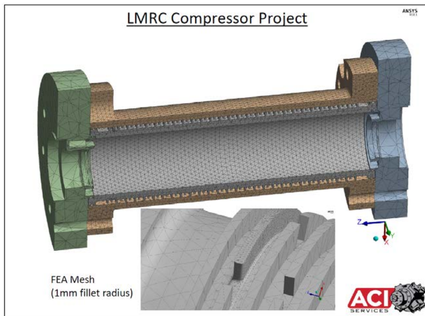
Figure 2. Meshed model of stator assembly housings
