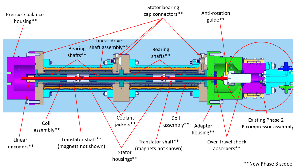
Figure 1. Cross-section of Phase 3 LMRC identifying major components
