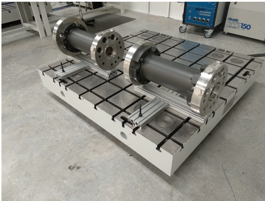
Figure 4. Photo of assembled motor stators
