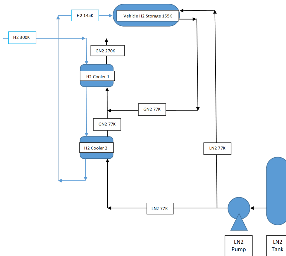
Figure 2. Cooling equipment configuration at a hydrogen refueling station that requires LN 2 temperature cooling of both hydrogen gas and onboard storage tank
