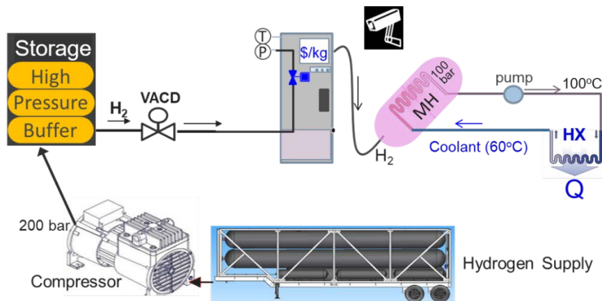
Figure 1. Hydrogen refueling station configuration for low-pressure (100 bar) and near-ambient-temperature dispensing
