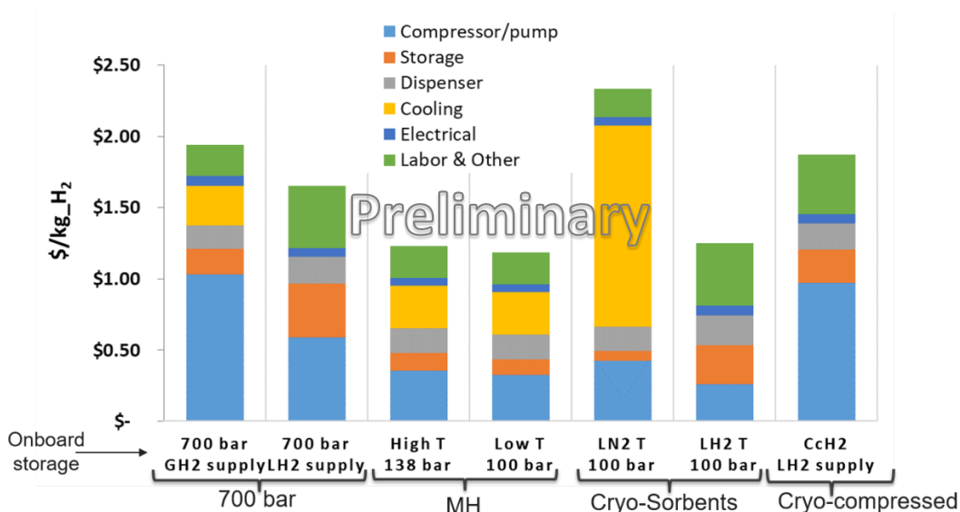
Figure 3. Impact of various FCEV onboard storage P and T requirements on the levelized cost of hydrogen fueling assuming gaseous tube trailer or liquid tanker delivery
