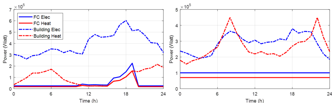
Figure 1. Fuel cell operation results in simulation with no additional battery or thermal storage (left: office; right: hotel)
