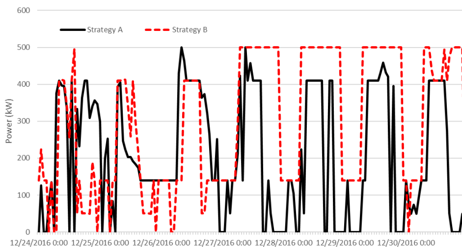
Figure 2. Fuel cell operation for the large office in Baltimore (WSU EAGERS approach)
