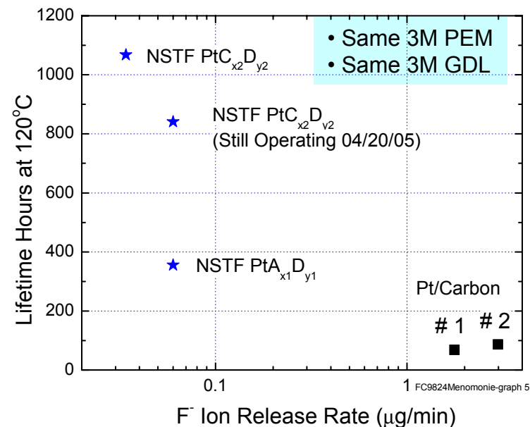
Lifetime versus F - ion release rate for NSTF and Dispersed Pt/C MEA's
