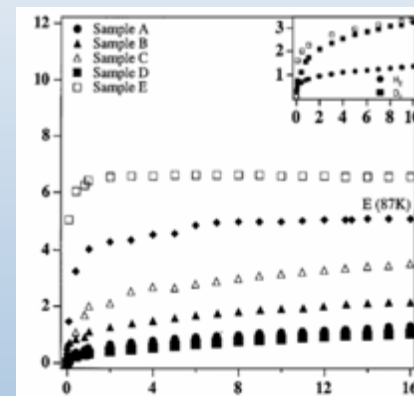
6 wt% on SWNTs at 77K, 2 bar Pradhan, et al., JMR 17, 2209 (2002)
