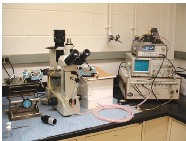
FIGURE 1. Apparatus for observing particle motion due to an applied electric field.
