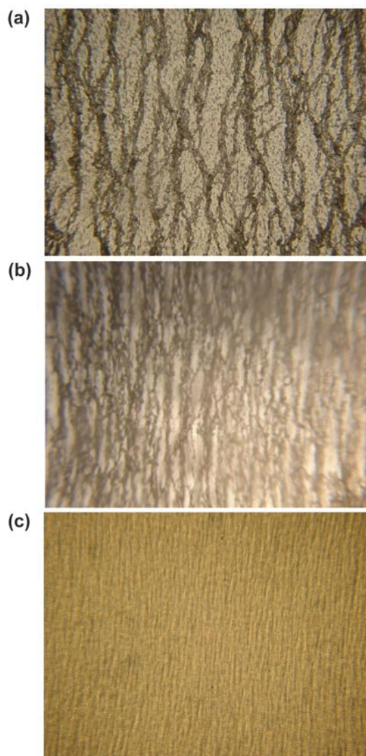
FIGURE 3. (a) 5 wt% Nafion ® in PVA, (b) 10 wt% SPEEK in PVA, and (c) 5 wt% sulfonated polystyrene in PVDF. In each case, particles are aligned in the direction of the field applied during solvent casting of the membrane.
