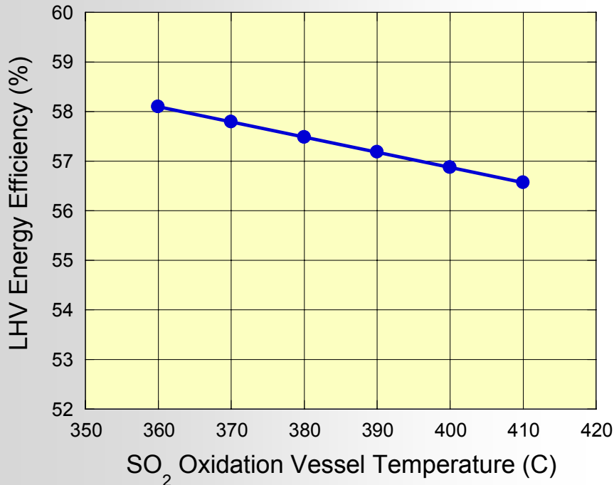
SO 2 Oxidation Temperature
