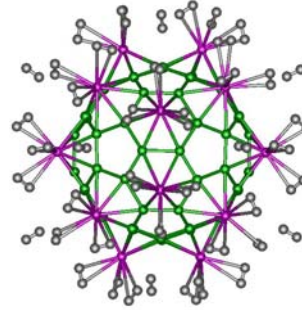
8.6 wt % \text{B}_{60}\text{Sc}_{20}\text{H}_{144}
