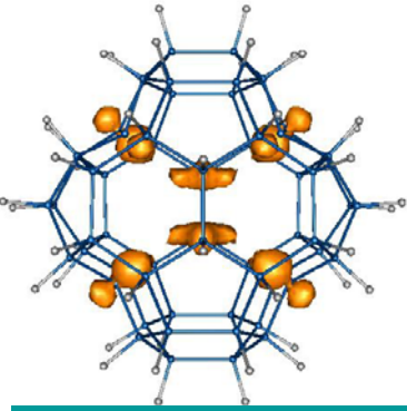
6.1 wt% \text{Ca}_2@C_{60}H_{52}
