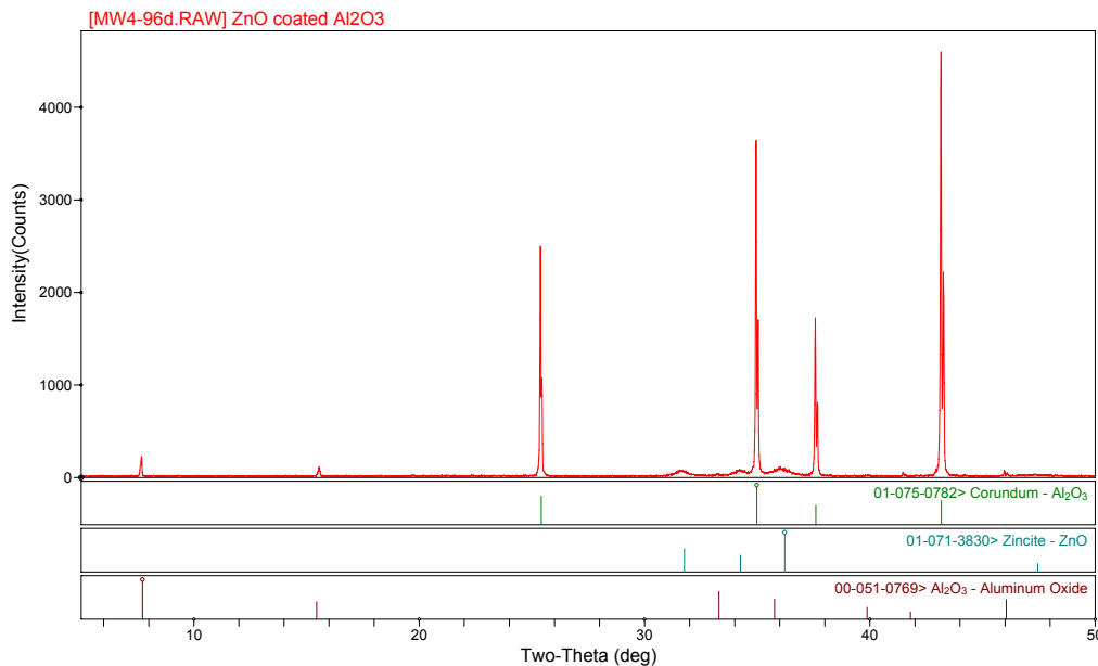
XRD showing Al 2 O 3 with small ZnO peaks
