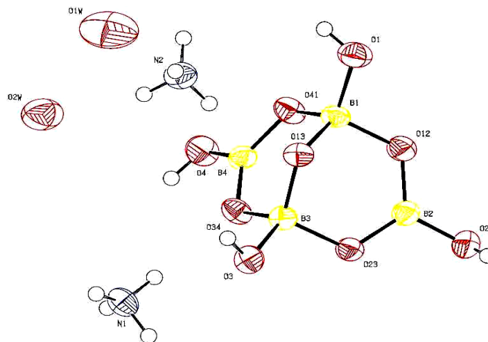
ORTEP diagram of \{[(\text{NH}_4)_2][\text{B}_4\text{O}_5(\text{OH})_4] \cdot 1.4\text{H}_2\text{O}\} at 50% probability
