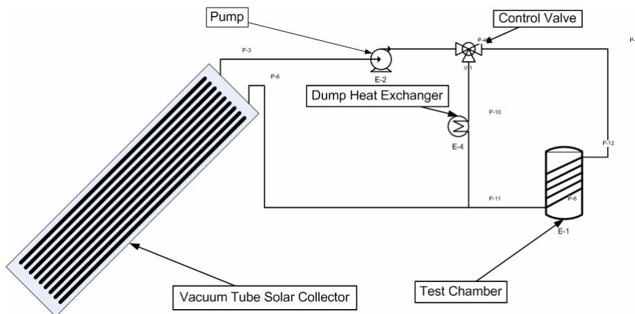
Current Solar Thermal Test System
