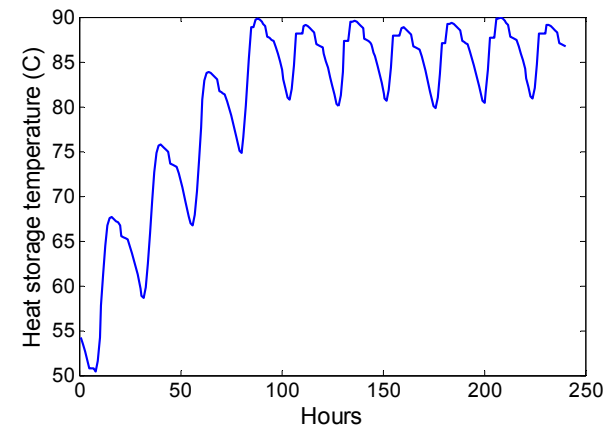
Thermal Response of Full Size System With Thermal Storage and Heat For Ancillary Purposes
