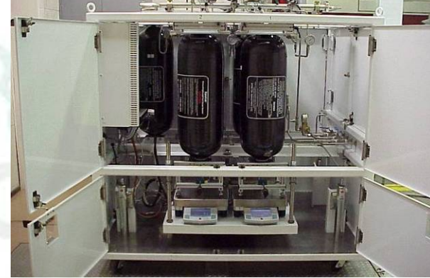
Hydrogen Mass Flow Measurement (Fuel Economy)
