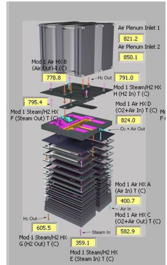
Heat Recuperator (1 of 3)
