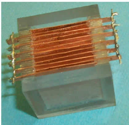
Metal-Insulator-Metal capacitor bank (left) and enclosure vessel with electrical leads (right) used in proof-of-concept experiments.
