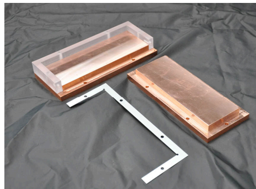
Parallel Plate Capacitor. (Left) test apparatus is shown disassembled showing copper plates, acrylic body and conductive shims. (Right) Assembled test apparatus with top removed. Close inspection shows thin test aperture where porous absorbent is placed for testing.
