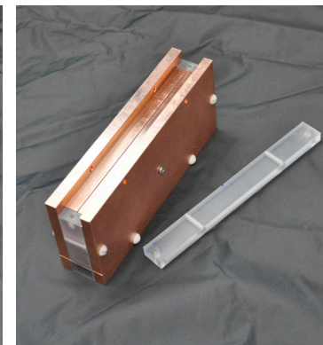
Parallel Plate Capacitor. (Left) test apparatus is shown disassembled showing copper plates, acrylic body and conductive shims. (Right) Assembled test apparatus with top removed. Close inspection shows thin test aperture where porous absorbent is placed for testing.
