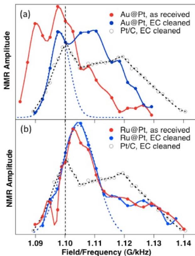
FIGURE 3. in situ ^{195}\text{Pt} NMR spectra (area-normalized) of Au@Pt (a) and Ru@Pt (b) NPs for as-received (red) and EC-cleaned (blue) samples. The black open circles and dashed line are the spectrum of a 2.5 nm pure Pt/C sample for reference. The vertical dashed line indicates the spectral position of surface Pt atoms for clean pure Pt/C NPs.
