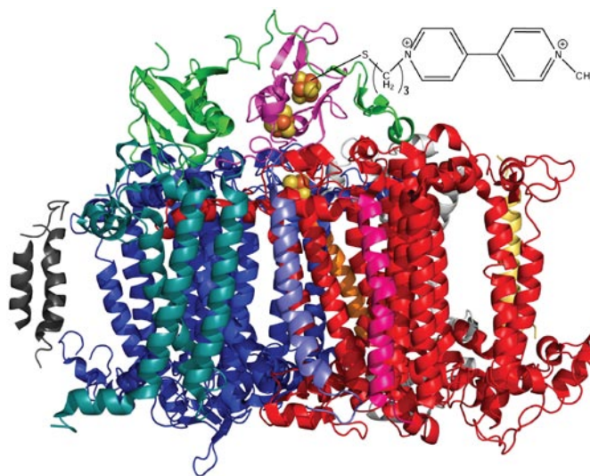
FIGURE 1. Depiction of the PS I—1-(3-thiopropyl)-1'-(methyl)-4,4'-bipyridinium construct. The electron transfer cofactors F_X , F_A , and F_B (from bottom to top) are shown as spheres within the protein scaffold. The molecular wire is attached at the F_B cluster, located inside the PsaC subunit (pink). The PsaD subunit (green) resides on top of the membrane spanning portion and adjacent PsaC. The TPMBP moiety is not drawn to scale.
