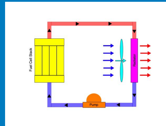
Dynalene FC Fuel Cell Cooling System
