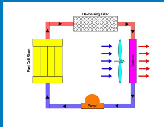
Typical DI Water Fuel Cell Cooling System
