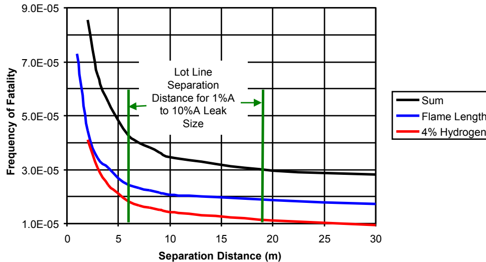
Total Risk - 15000 psig System
