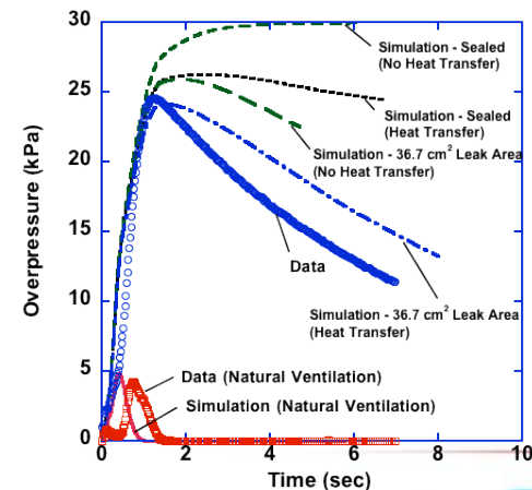
Comparison of Simulation and Data for Ign. Deflagration Overpressure
