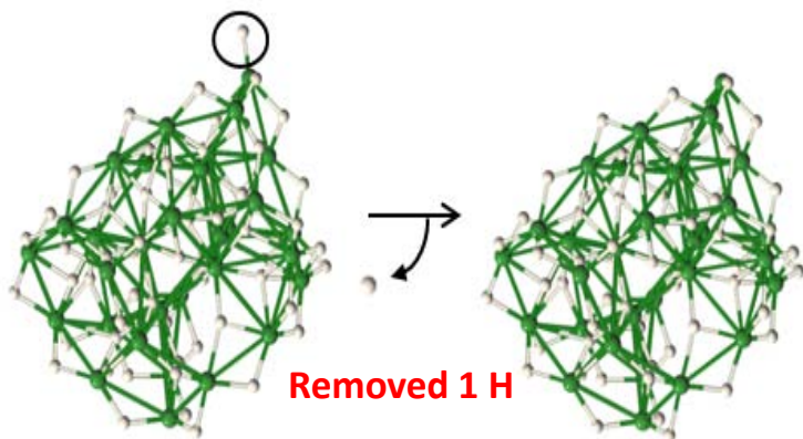
Mg 31 H 62 amorphous nanoparticle H bonded to 1 Mg atom
