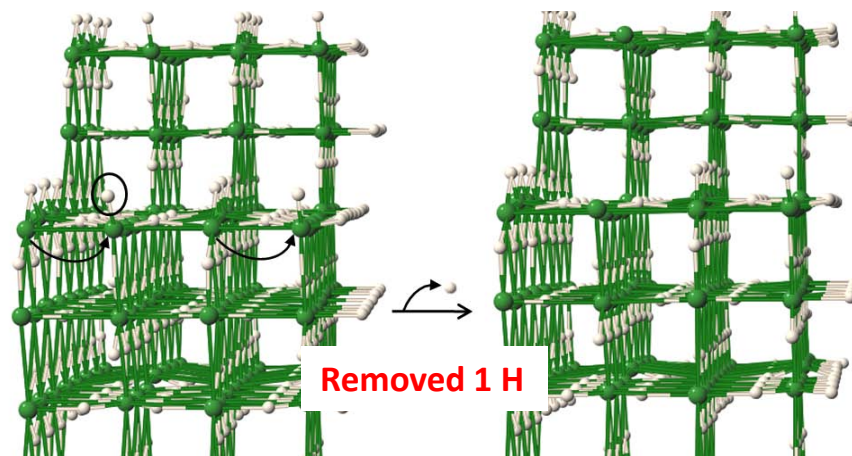
Bulk MgH 2 (110) Surface with (001) Steps H bonded to 1 Mg step-edge atom
