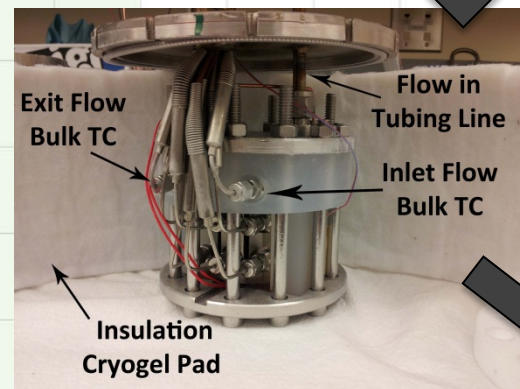
Assembled view of the test section
