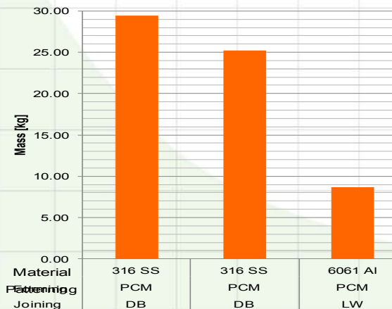
System Mass by Design
