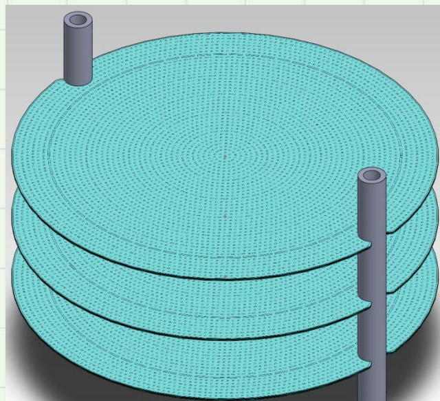
30 cm MATI Concept
