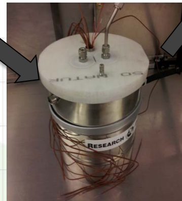
Test section dewar
