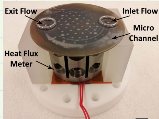
Partially assembled view of the test section
