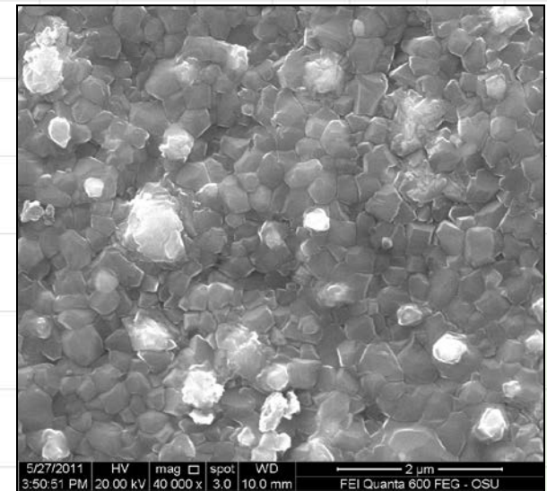
SEM of Wet Deposited Catalyst
