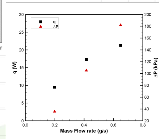
Preliminary heat transfer test with N 2 gas
