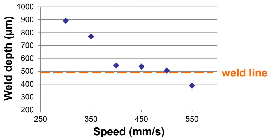
Weld depth vs Weld speed Power = 1000 W
