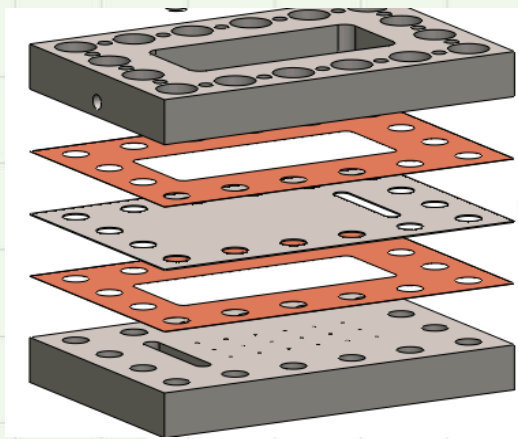
Exploded View of Combustor test article
