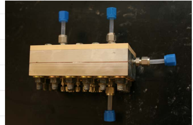
Assembled Test Section
