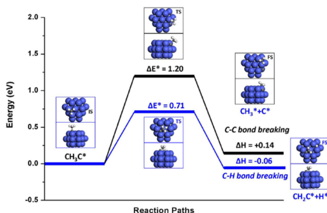
FIGURE 2. The C-H bond-breaking of CH_3C^* is more favorable than the C-C bond-breaking, indicating the CH_3 formation is least likely.
