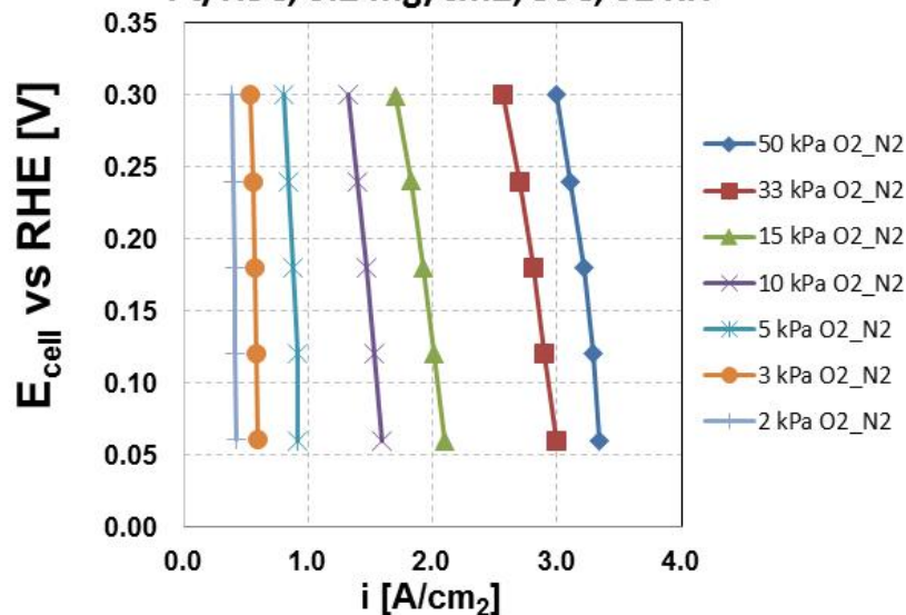
Pt/HSC, 0.2 mg/cm 2 , 80C, 62 RH
