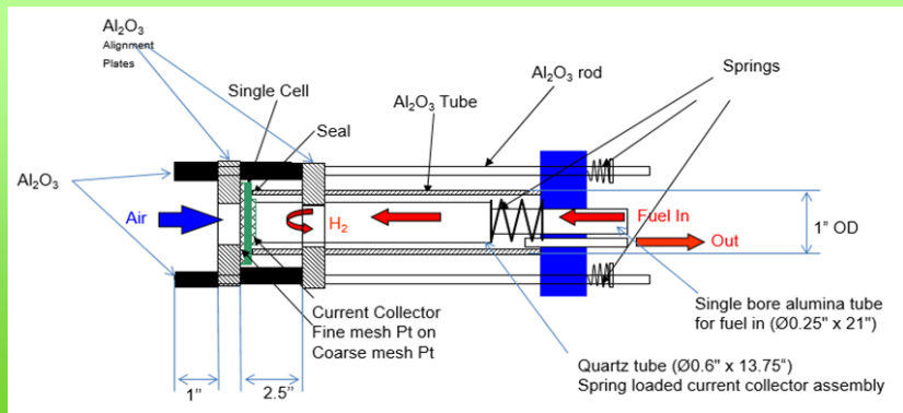
Schematic of the all alumina button cell test stand used at SG
