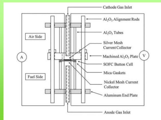
Schematic of the button cell test stand used at BU
