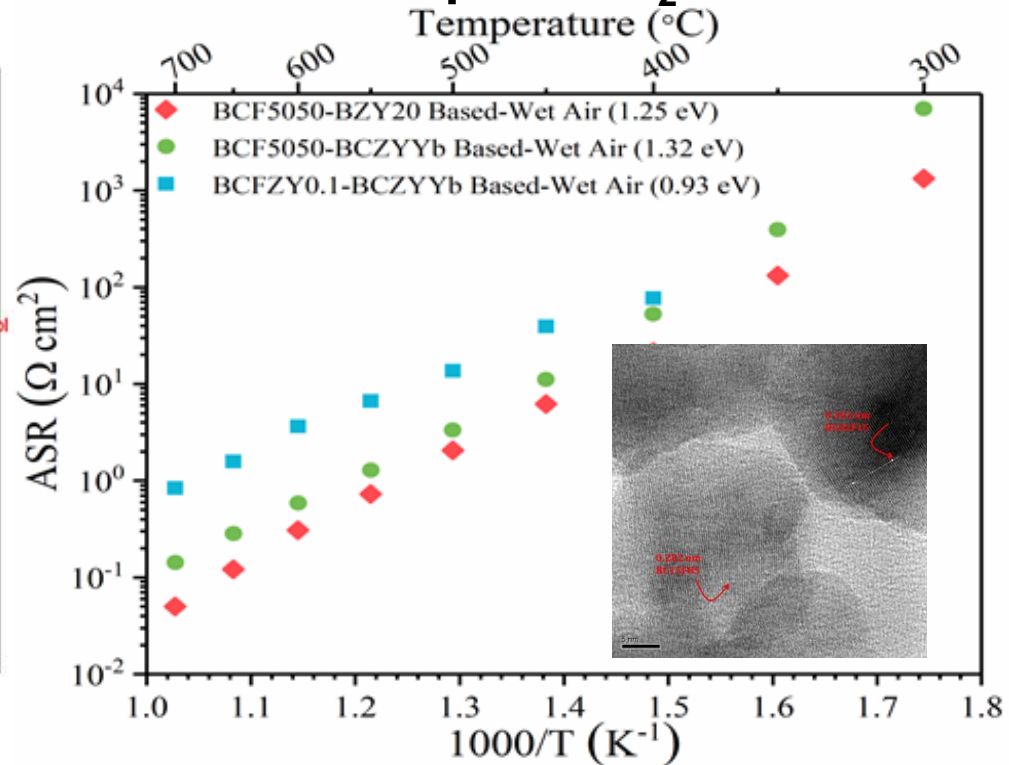
Performance of BCF nanocomposite oxygen electrode based on symmetrical cells.
