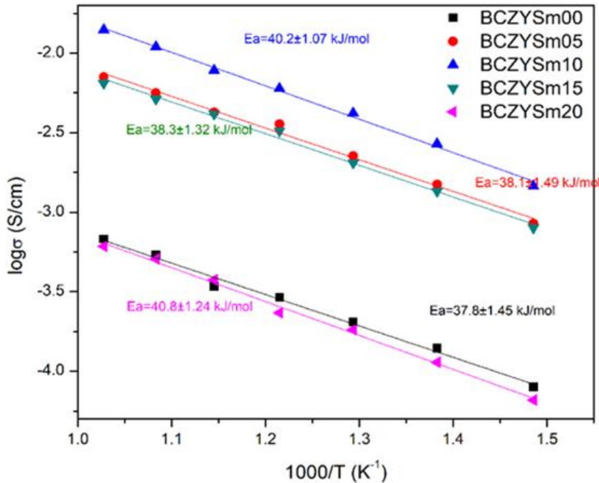
Total conductivity VS temperature in wet 5% H 2
