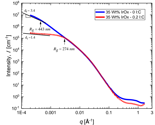
USAXS of Concentrated Ink
