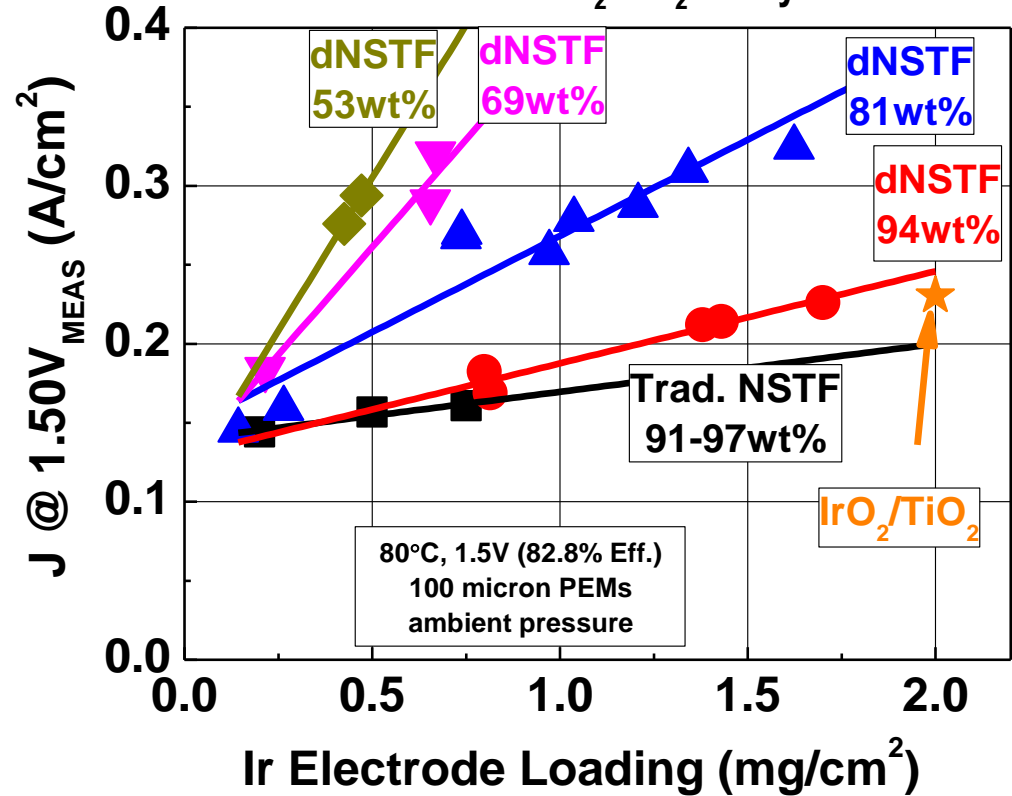
OER Activity vs. Electrode Type, Ir wt% Ir/NSTF or IrO 2 /TiO 2 catalysts
