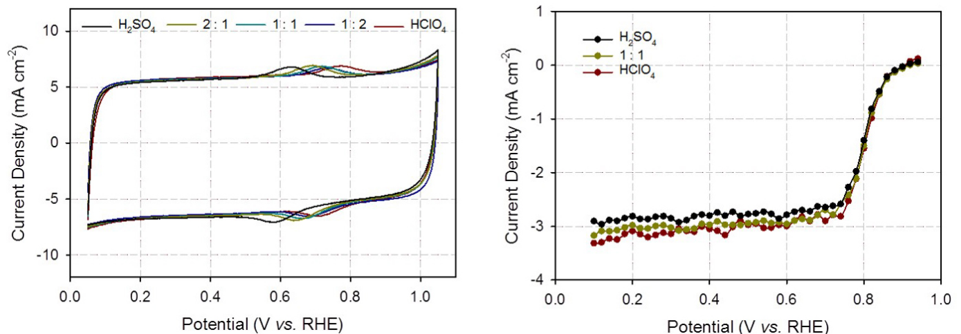
FIGURE 2. Left graph shows cyclic voltammograms for different mixtures of \text{H}_2\text{SO}_4 and \text{HClO}_4 ; right graph compares ORR for \text{H}_2\text{SO}_4 , \text{HClO}_4 , and a 50% mixture of the two
