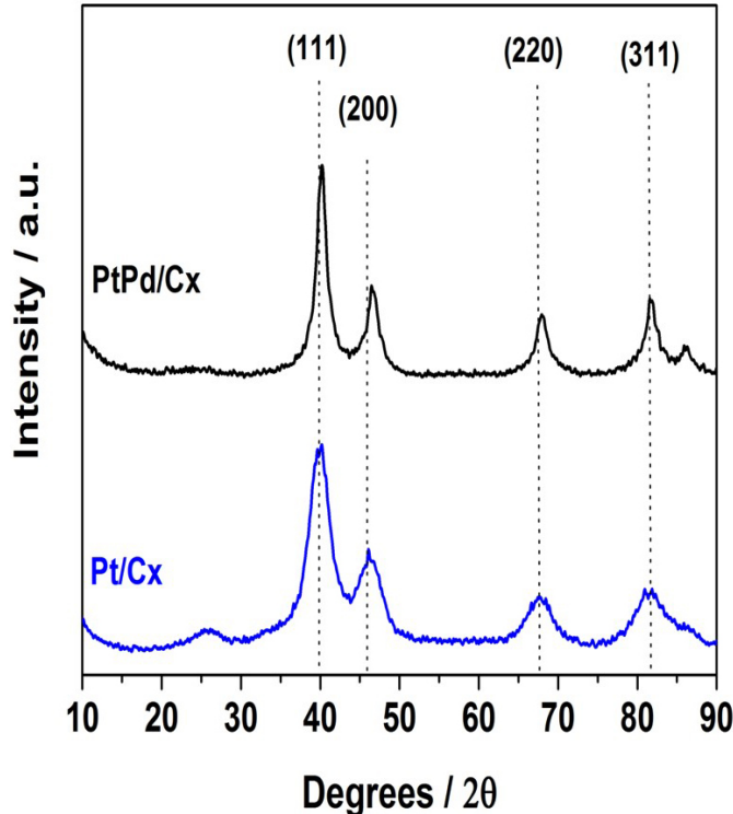
FIGURE 1. X-ray diffraction results of Blue-O Technology catalyst samples
