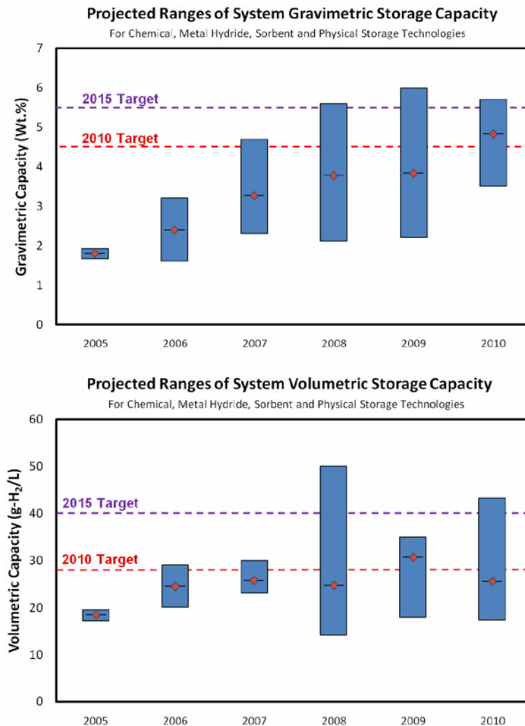
FIGURE 1. Estimates of gravimetric and volumetric capacities projected for on-board storage systems that can supply 5.6 kg of usable hydrogen as compared to DOE targets (based upon engineering analyses). Note that the plotted data points are the average values for all systems analyzed during each year while the bars correspond to the range of maximum and minimum values obtained in each year. Also note that systems with predicted capacities exceeding the gravimetric or volumetric targets do not meet other targets.
